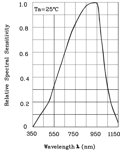
Fig.2 Spectral Sensitivity
