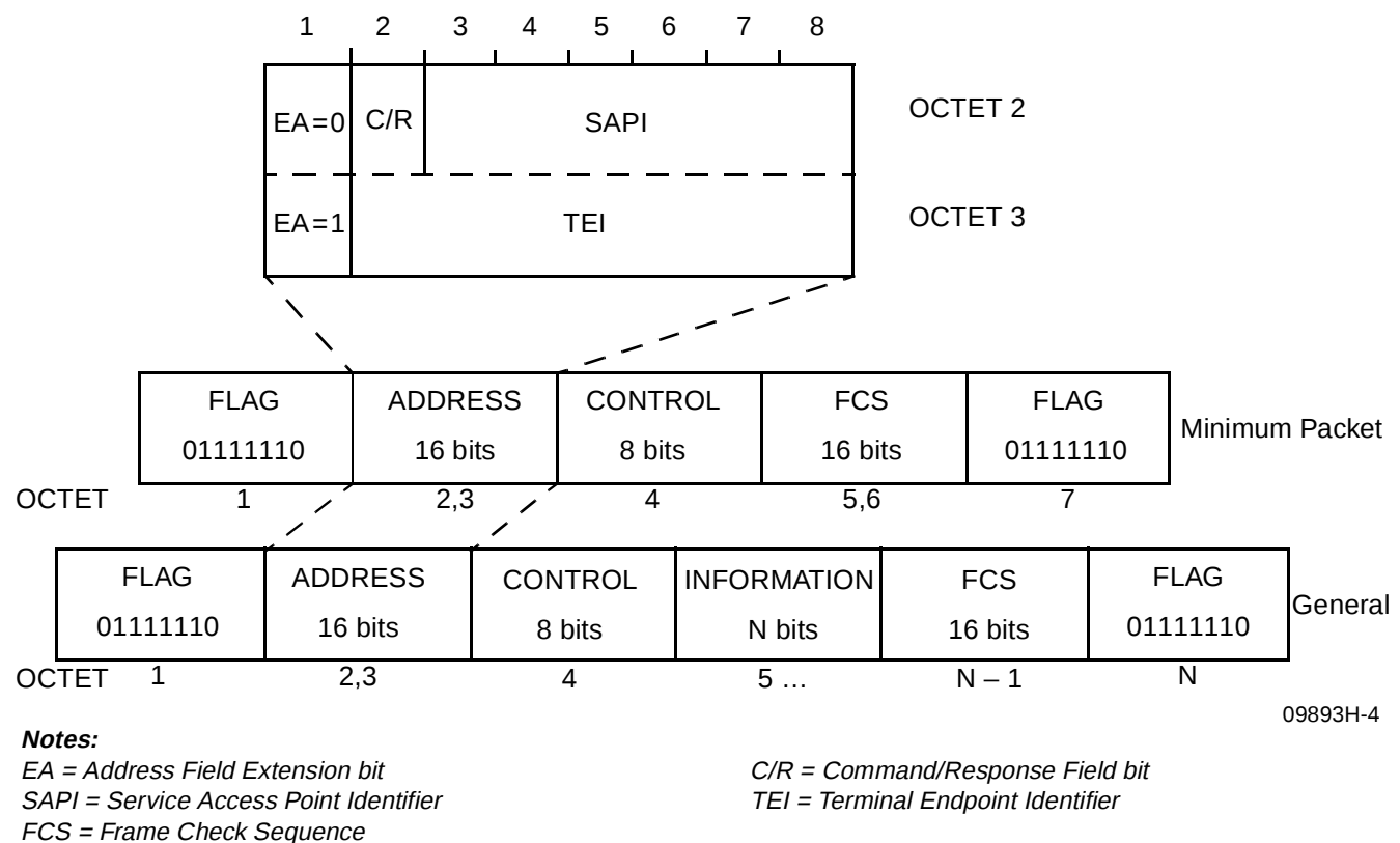
Figure 4. Level-2 Frame Structure Formats
