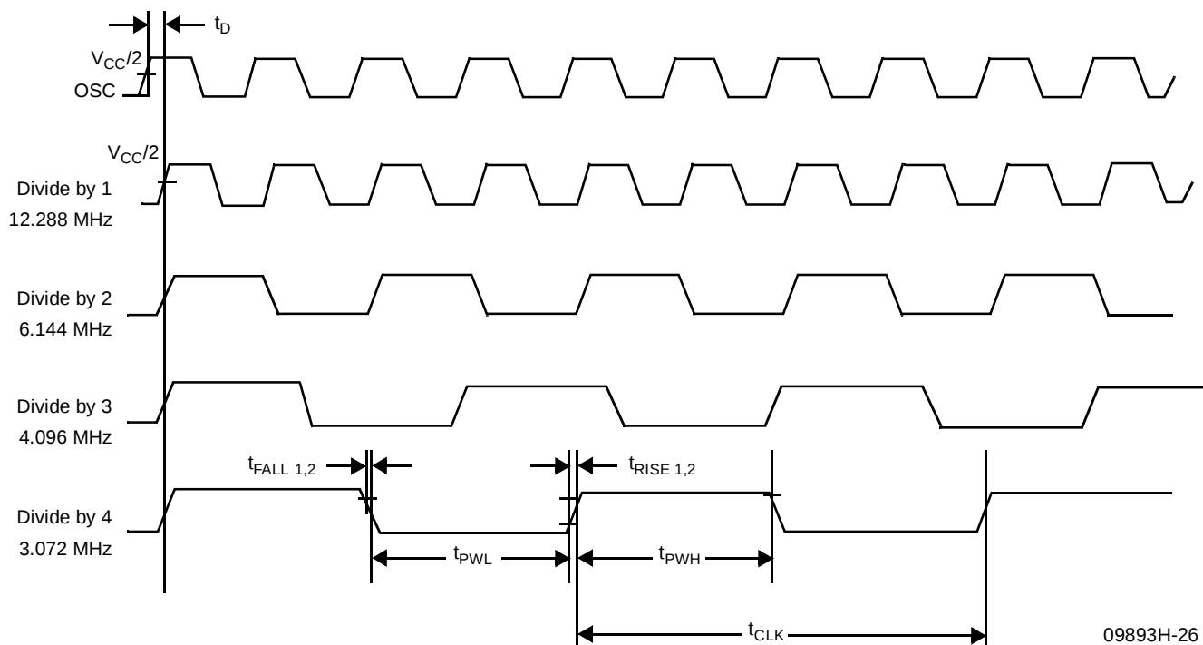
Figure 34. OSC/MCLK Timing
