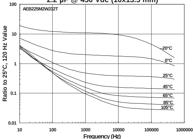
ESR vs Temperature and Frequency 2.2 \mu F @ 450 Vdc (10x13.5 mm)
