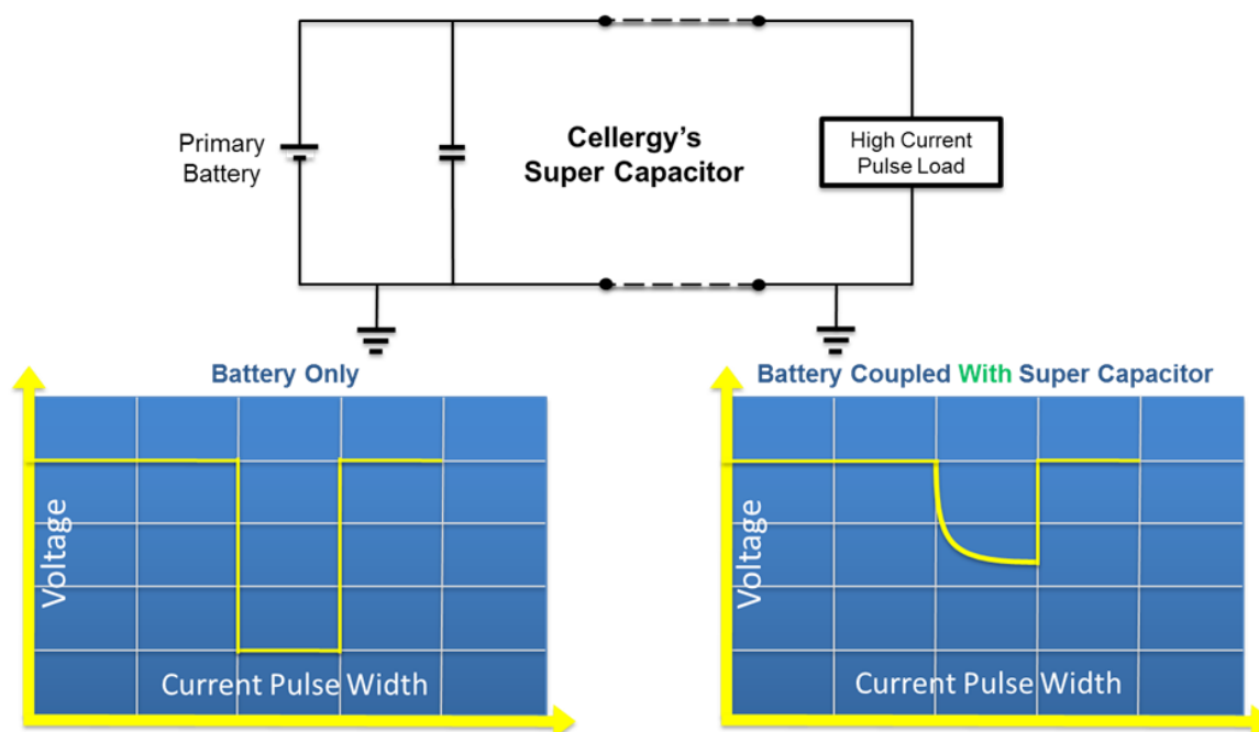
Figure 4: Basic Battery + Supercapacitor Electrical Scheme
