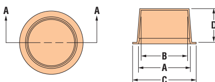
TAPERED CAP
