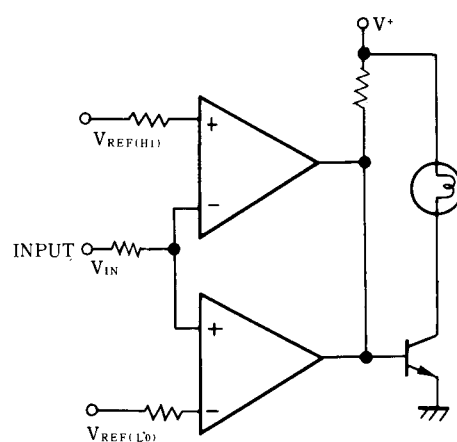
Limit Comparator
