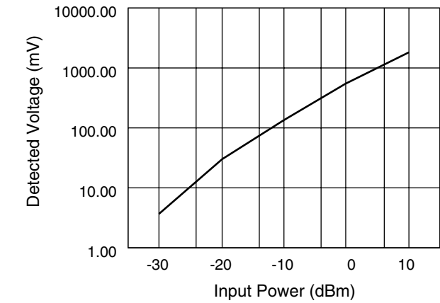
Typical Detector Characteristics @ 1.8 GHz
