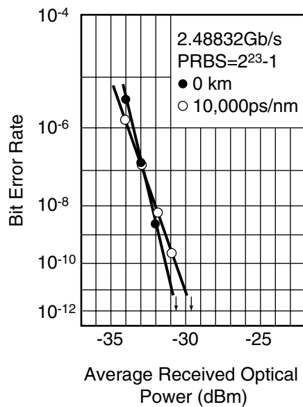
Fig. 8 Transmission Characteristics
