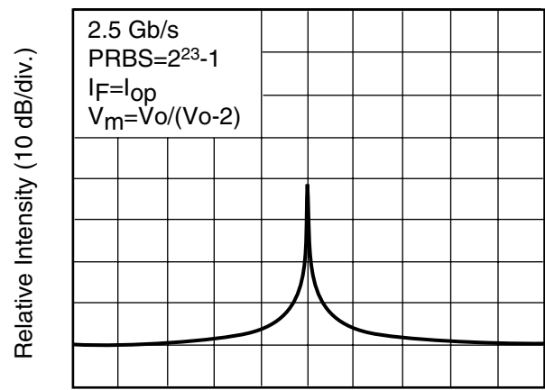
Fig. 2 Lasing Spectrum
