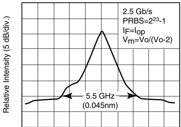
Fig. 1 Lasing Spectrum
