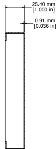
SECTION EE-EE
