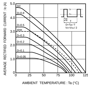
Fig.8 Derating curve ( I_o - T_a ) (when mounted on glass epoxy PCBs)
