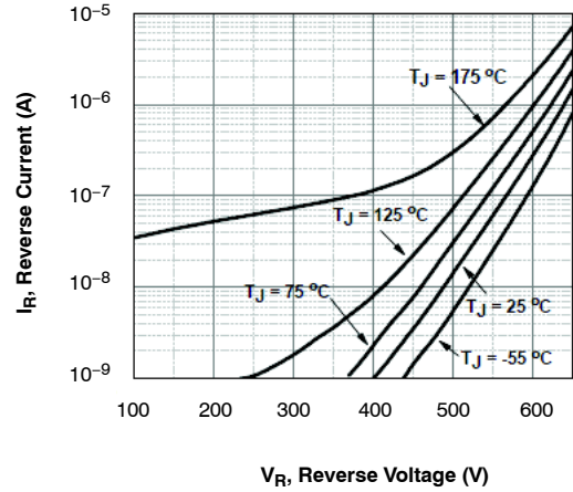
Figure 2. Reverse Characteristics
