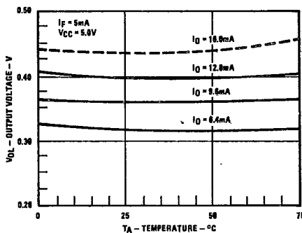
Figure 3. Output Voltage, V_O , vs Temperature and Fan-Out
