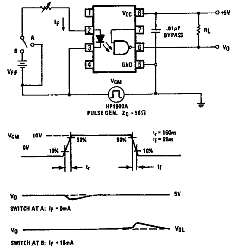
Figure 12. Test Circuit for Transient Immunity and Typical Waveforms
