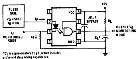
Figure 7. Test Circuit for t_{PHL} and t_{PLH} (6N137 Only)
