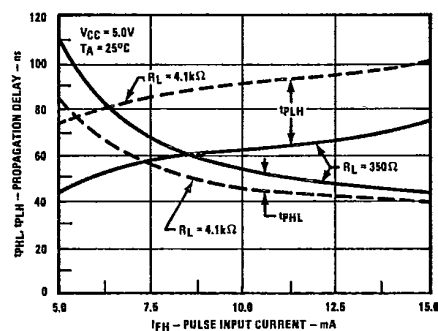
Figure 8. Propagation Delay, t_{PHL} and t_{PLH} vs Pulse Input Current, I_{FH}
