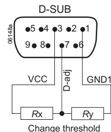
Fig. 19 Wiring to adjust both threshold levels of option D1 or D5
