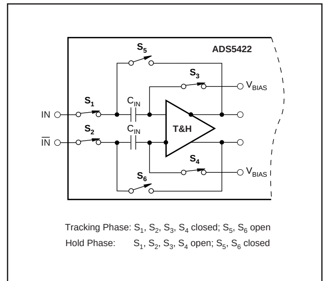
FIGURE 1. Simplified Circuit of Input Track-and-Hold Amplifier.
