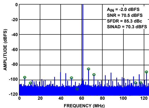
FIGURE 19. SINGLE-TONE SPECTRUM AT 190MHz (250MSPS)
