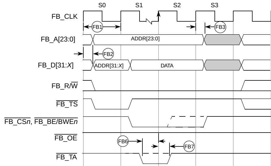
Figure 15. Flexbus Write Timing
