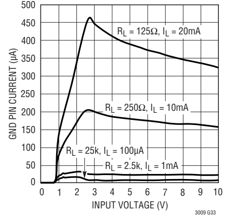
GND Pin Current LT3009-2.5
