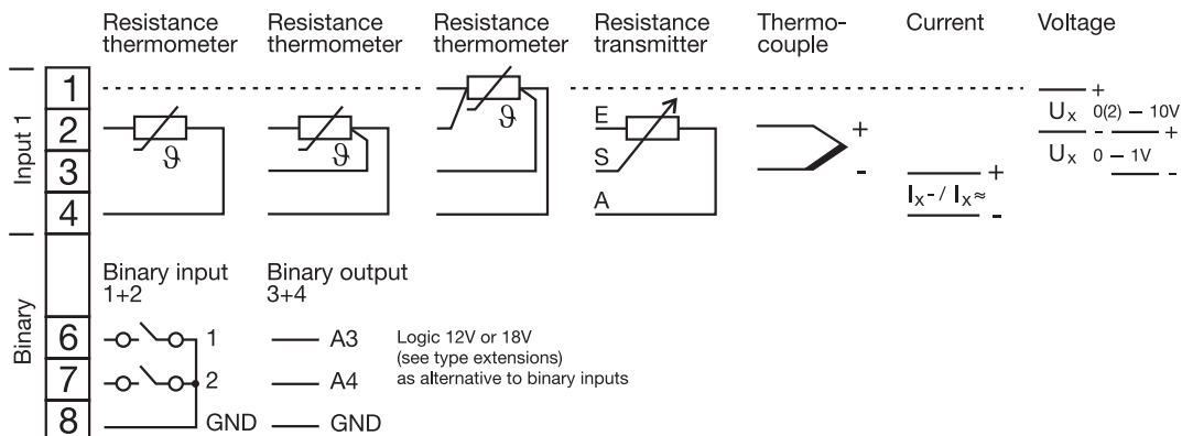
Terminal strip 2
