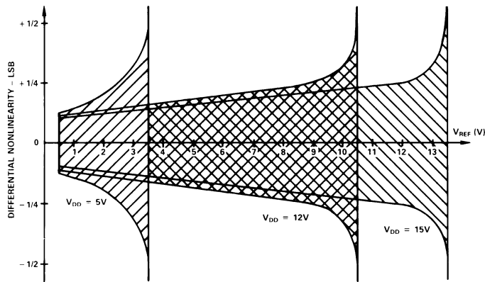
Figure 3. Differential Nonlinearity vs. V_{REF}
