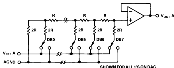
Figure 7. D/A Simplified Circuit Diagram
