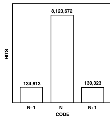
TPC 21. "Grounded-Input" Histogram (Input Span = 2 V p-p)
