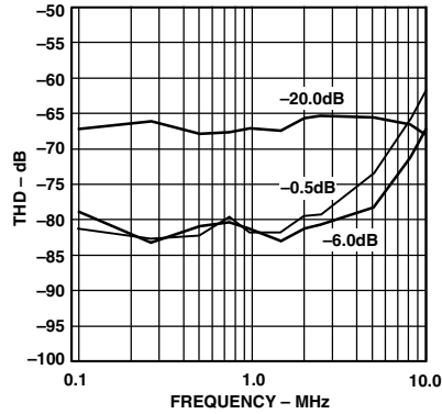
TPC 14. THD vs. Input Frequency (Input Span = 2.0 V p-p, V_{\text{CM}} = 2.5 V)
