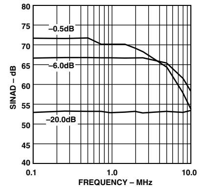
TPC 15. SINAD vs. Input Frequency (Input Span = 5.0 V p-p, V_{\text{CM}} = 2.5 V)
