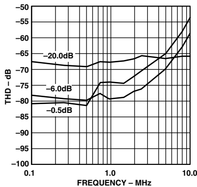
TPC 16. THD vs. Input Frequency (Input Span = 5.0 V p-p, V_{\text{CM}} = 2.5 V)
