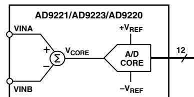
Figure 4. AD9221/AD9223/AD9220 Equivalent Functional Input Circuit
