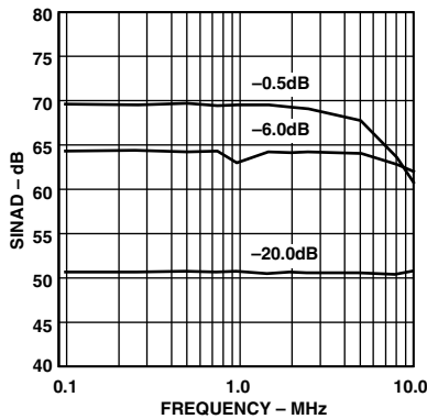
TPC 13. SINAD vs. Input Frequency (Input Span = 2.0 V p-p, V_{\text{CM}} = 2.5 V)
