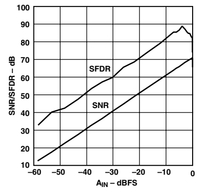
TPC 18. SNR/SFDR vs. A_{\text{IN}} (Input Amplitude) ( f_{\text{IN}} = 1.5 MHz, Input Span = 2 V p-p, V_{\text{CM}} = 2.5 V)
