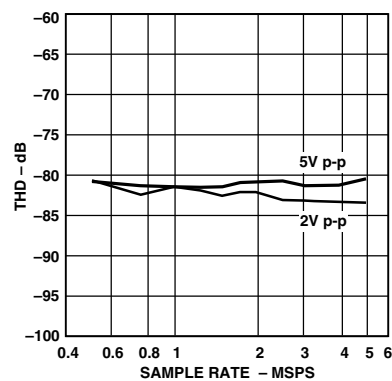
TPC 17. THD vs. Sample Rate ( A_{\text{IN}} = -0.5 dB, f_{\text{IN}} = 500 kHz, V_{\text{CM}} = 2.5 V)
