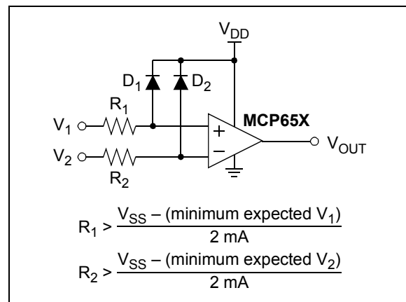
FIGURE 4-4: Protecting the Analog Inputs.
