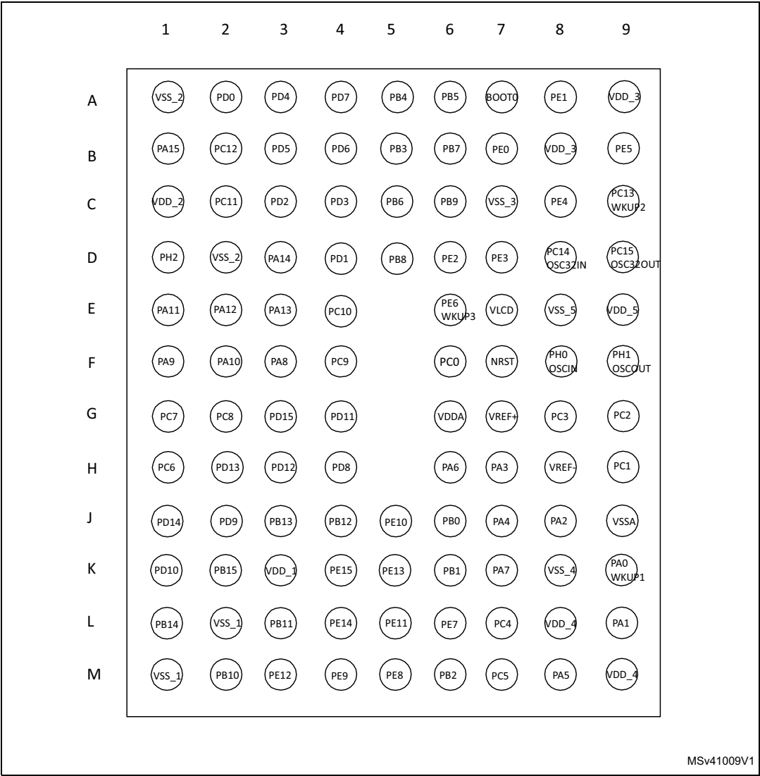
Figure 5. STM32L15xVEY WLCSP104 ballout
