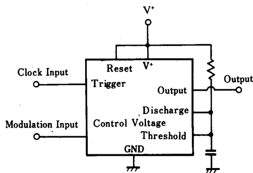
Pulse Width Modulation Circuit
