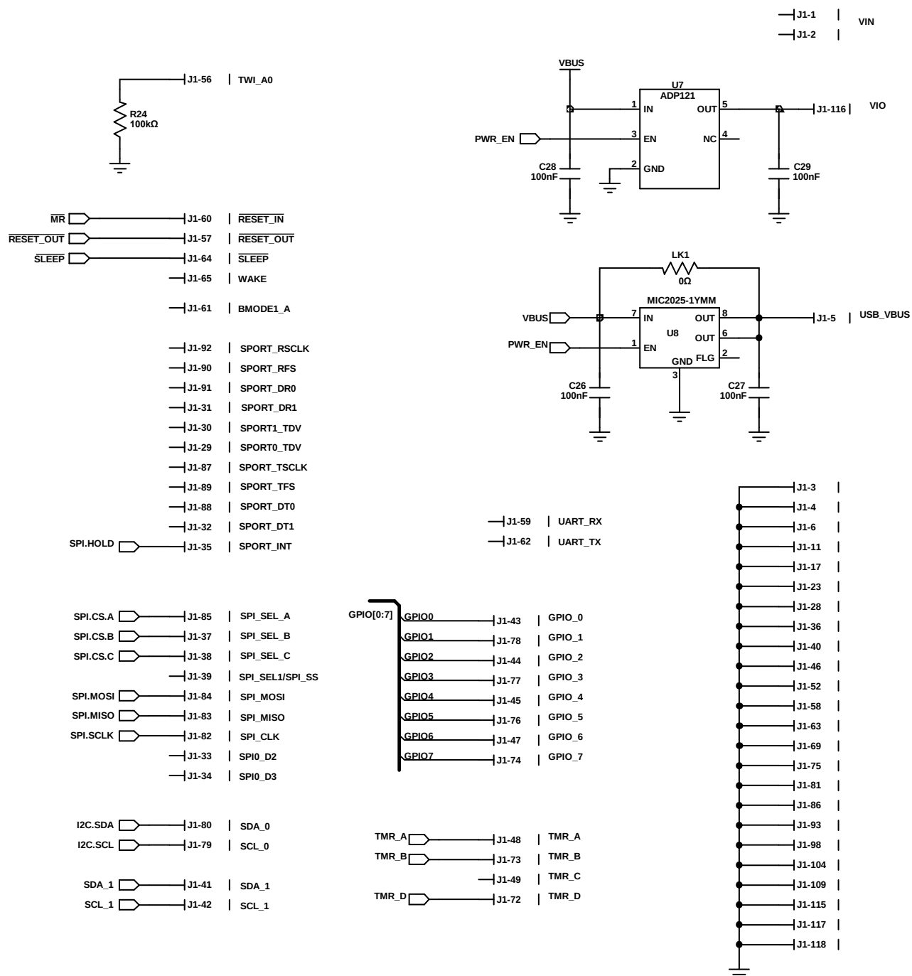
Figure 9. SDP-S—Connector
