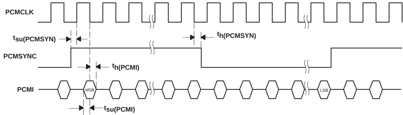
Figure 11. Receive Timing Diagram, 128 kHz
