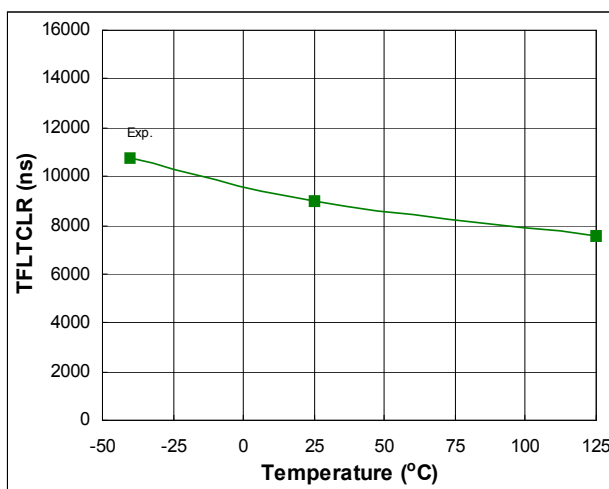
Fig. 48. FAULT Clear Time vs. Temperature
