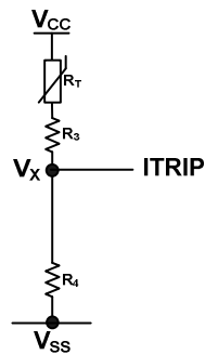
Figure 10: Programming over-temperature protection
