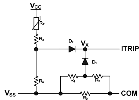
Figure 11: Using over-current protection and over-temperature protection
