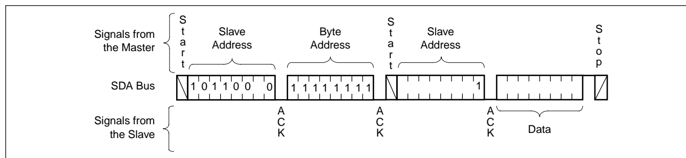
Figure 9. Read Sequence
