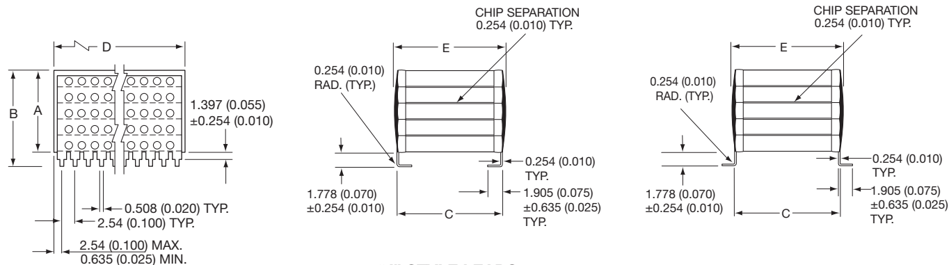
“J” STYLE LEADS
