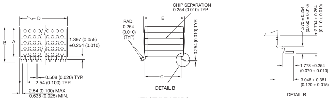
“Z” STYLE LEADS
