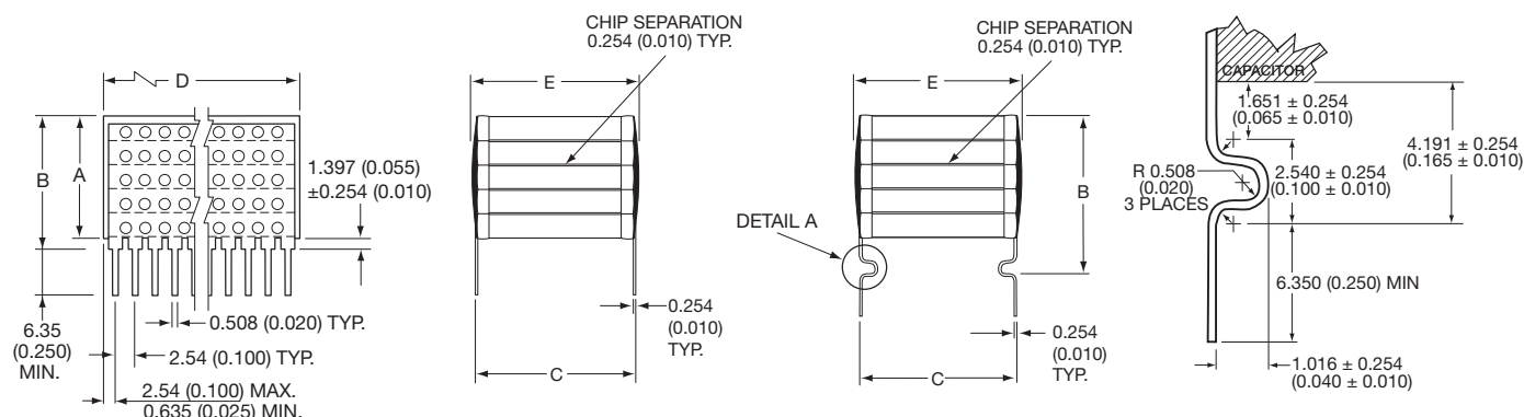
DETAIL A
