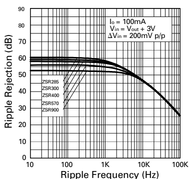
Ripple Rejection v Ripple Frequency
