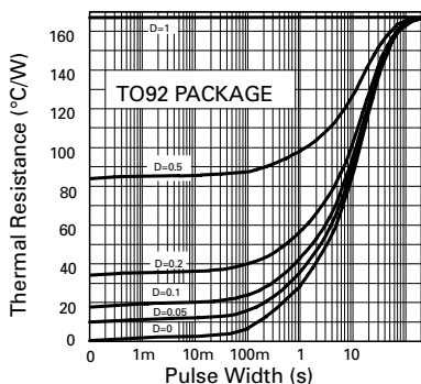
Thermal Resistance v Pulse Width
