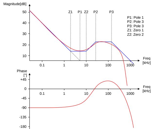
Figure 55. Transfer Function of PWM
