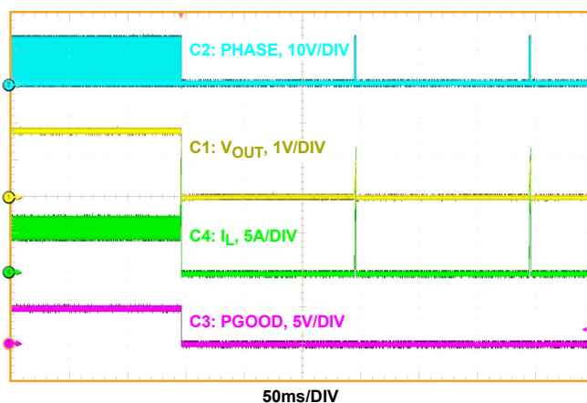
FIGURE 27. HICCUP OCP ( V_{IN} = 12V , V_{OUT} = 1.8V , 600kHz)
