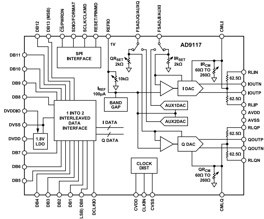
Figure 84. Simplified Block Diagram
