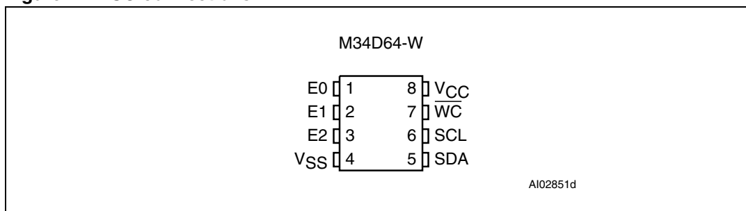
Figure 2. SO connections
