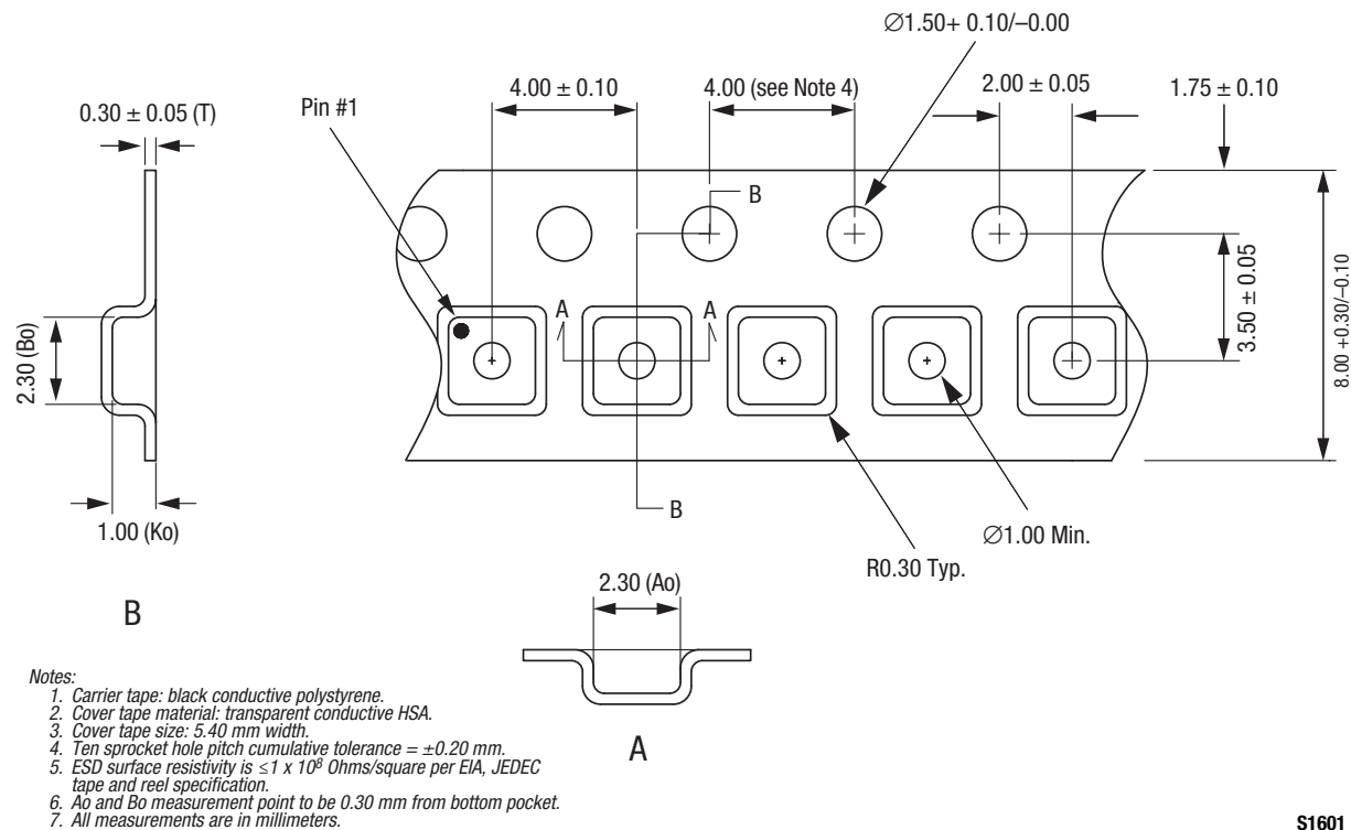
Figure 20. SKY67100-396LF Tape and Reel Dimensions
