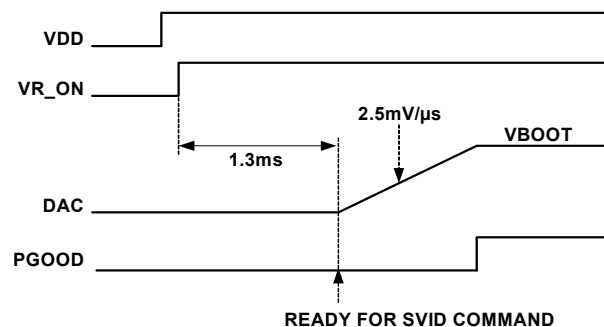
FIGURE 8. SOFT-START WAVEFORMS
