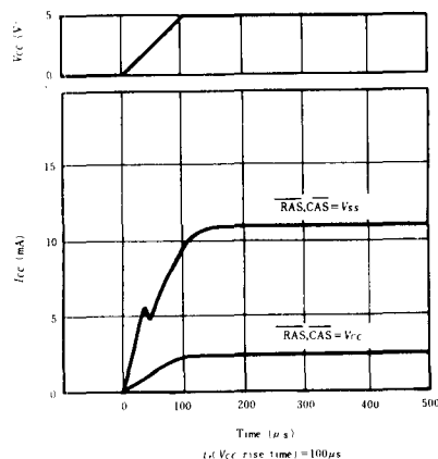
Fig.1 I_{CC} vs. V_{CC} during power up.
