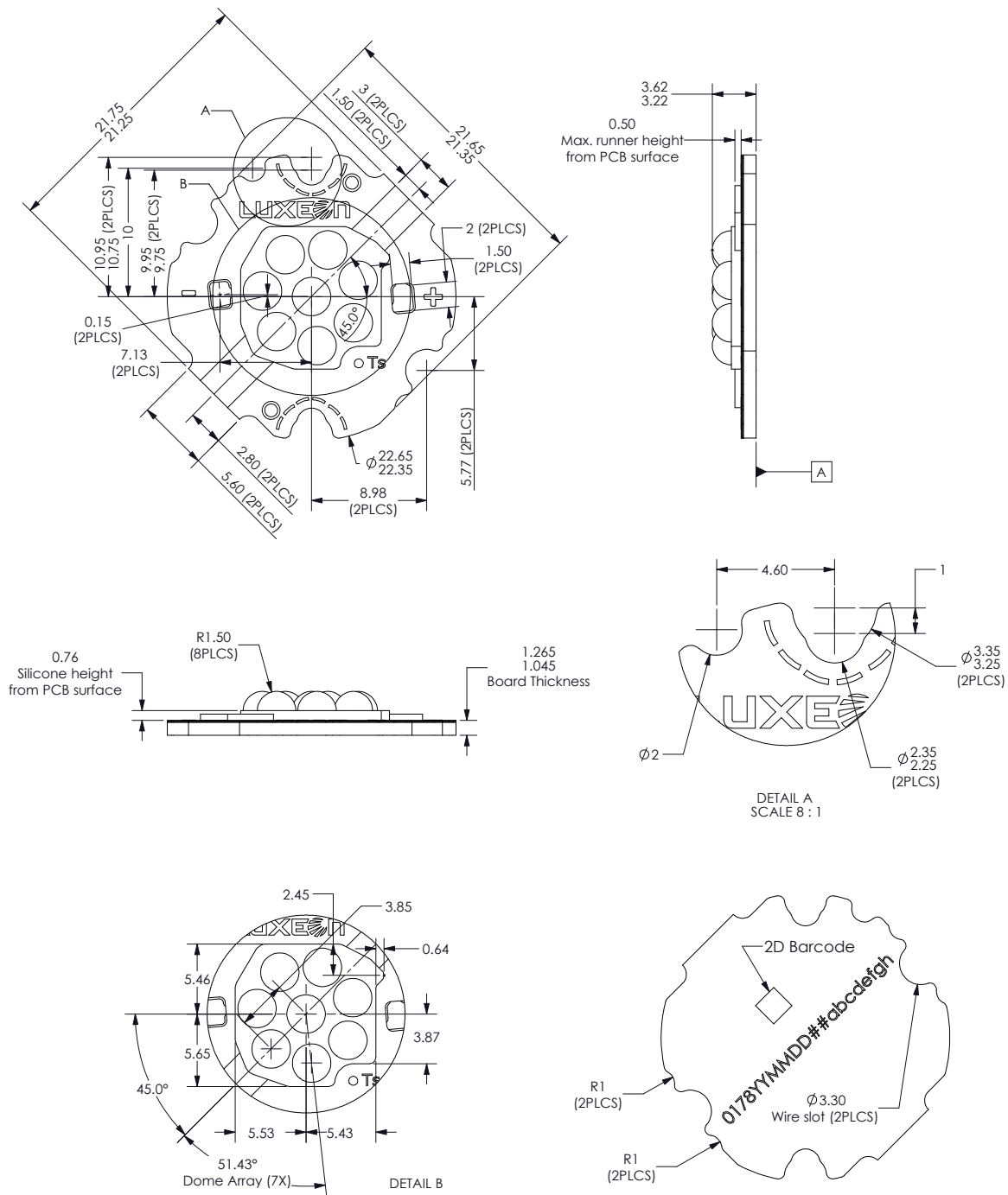
Figure 4. Dimensions for LXKx-Pxxx-xxx8(A).
