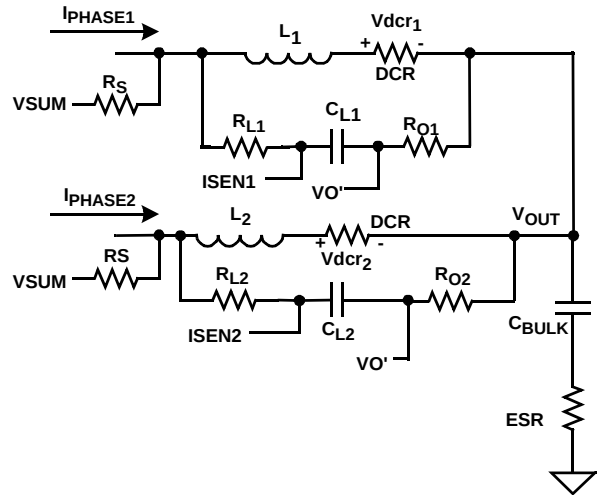
FIGURE 37. SIMPLIFIED SCHEMATIC FOR DROOP AND DIE SENSING WITH INDUCTOR DCR CURRENT SENSING
