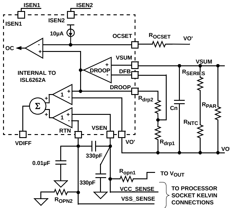
FIGURE 37. SIMPLIFIED SCHEMATIC FOR DROOP AND DIE SENSING WITH INDUCTOR DCR CURRENT SENSING
