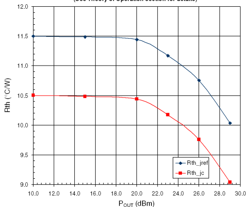
UMTS V_{CC}=8V and I_{REF}=60mA , R_{th} versus P_{OUT} @ 85°C Ambient (See Theory of Operation section for details)
