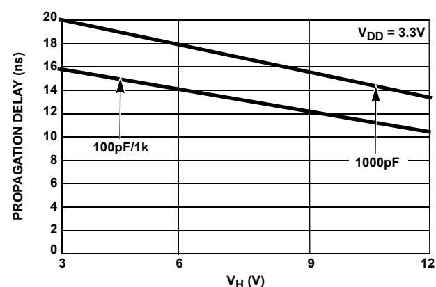
FIGURE 27. t_{pdF} vs V_H
