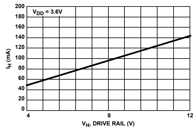
FIGURE 11. OPERATING I_H vs V_H AT 50MHz (NO LOAD)
