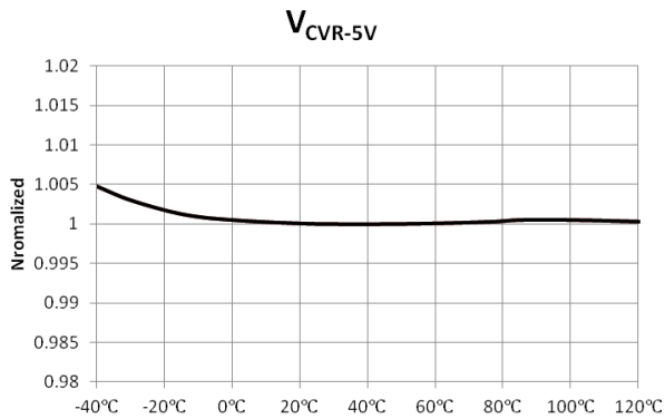
Figure 5 Reference Voltage at 5 V ( V_{CVR-5V} ) vs. Temperature
