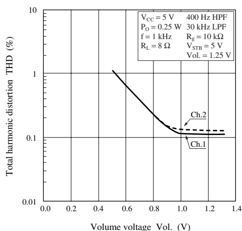
THD — Vol.
