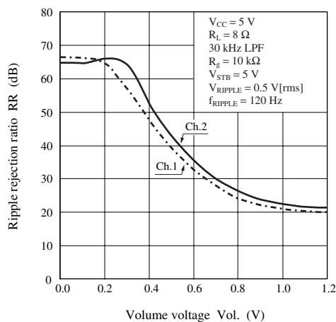
RR — Vol.
