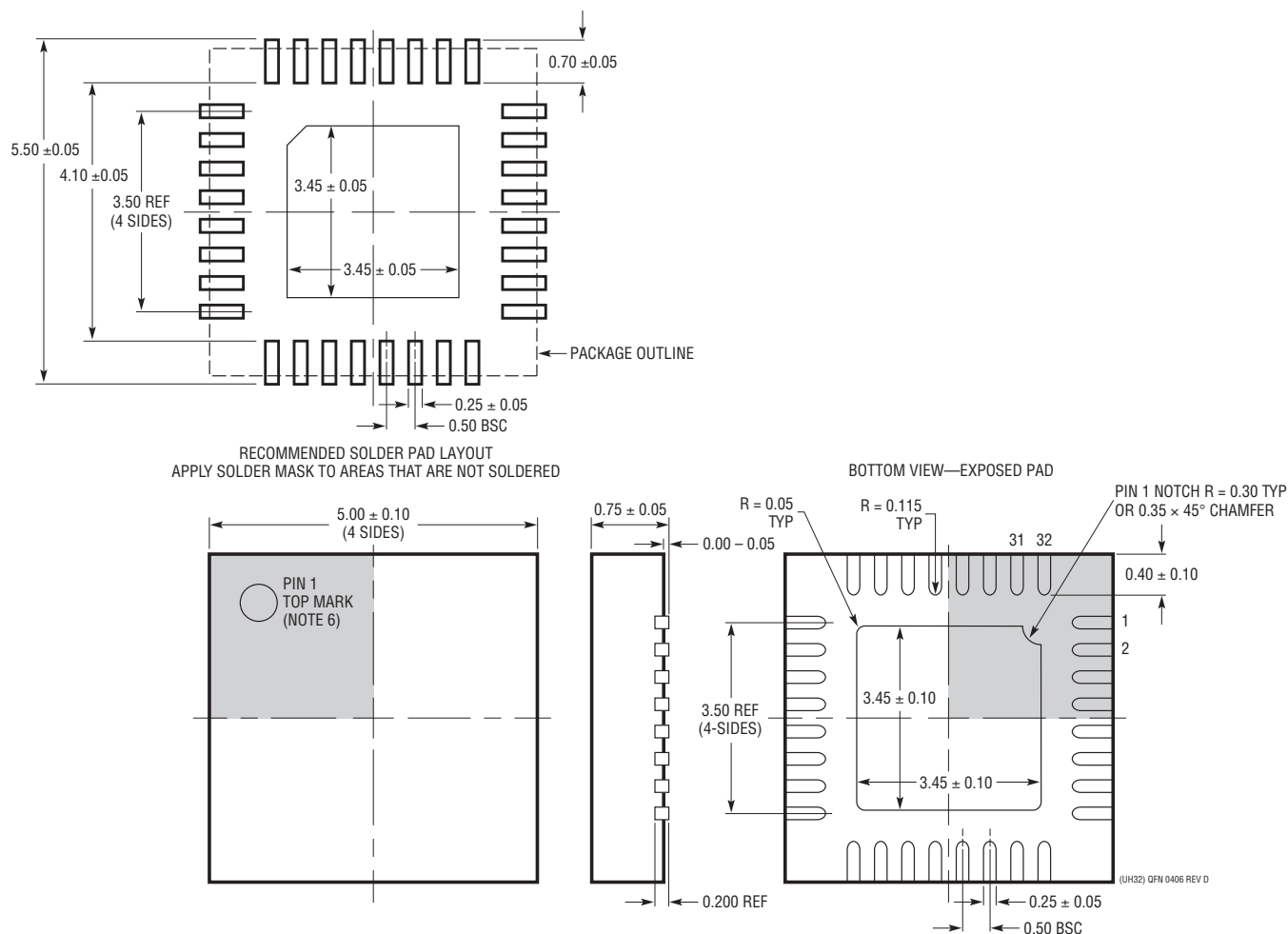
UH32 Package 32-Lead Plastic QFN (5mm × 5mm) (Reference LTC DWG # 05-08-1693 Rev D)
