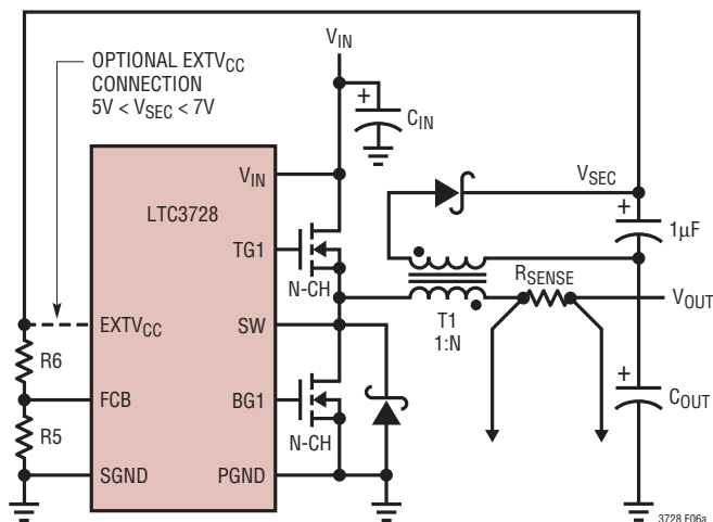
Figure 6a. Secondary Output Loop and EXT CC Connection
