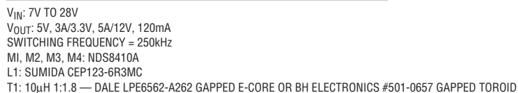
Figure 12. LTC3728 High Efficiency Low Noise 5V/3A, 3.3V/5A, 12V/120mA Regulator
