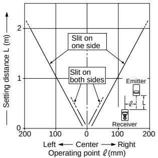
Parallel deviation with round slit masks ( \phi 2\text{mm} )
