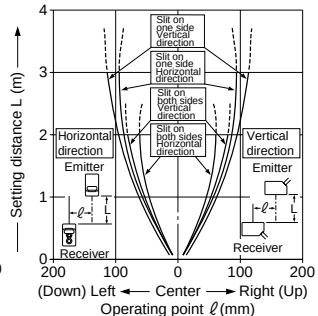
Parallel deviation with rectangular slit masks ( 2 \times 6\text{mm} )
