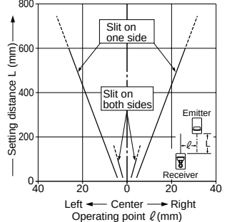
Parallel deviation with round slit masks ( \phi 1\text{mm} )
