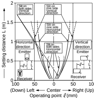
Parallel deviation with rectangular slit masks ( 0.5 \times 6\text{mm} )
