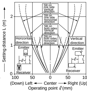
Parallel deviation with rectangular slit masks ( 1 \times 6\text{mm} )
