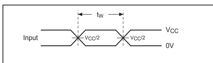
Voltage Waveforms Pulse Duration
