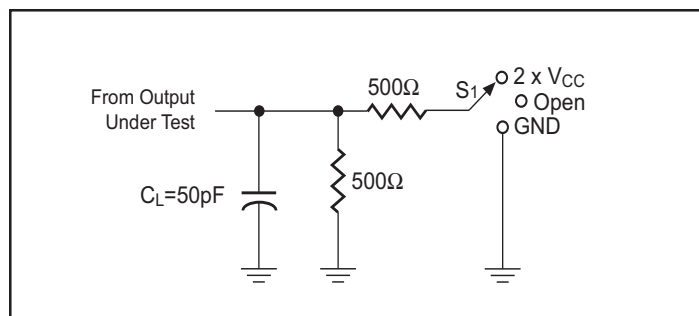
Load Circuit
