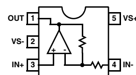
EL5197 (5 LD SOT-23) TOP VIEW
