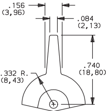
J2 LEVER
