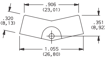
J3 ROCKER
