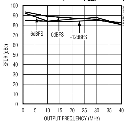
SPURIOUS-FREE DYNAMIC RANGE vs. OUTPUT FREQUENCY ( f_{CLK} = 100MHz )
