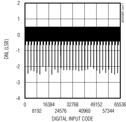
DIFFERENTIAL NONLINEARITY
