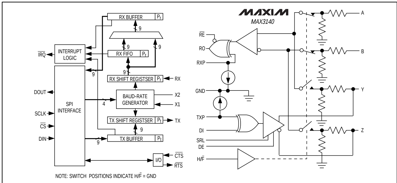
Figure 10. Functional Diagram
