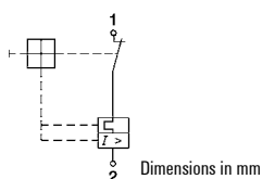
Internal Wiring Diagram
